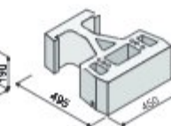
Geostone GWS III. FLAT
