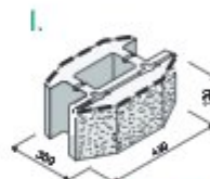
Geostone GWS I. BENT
